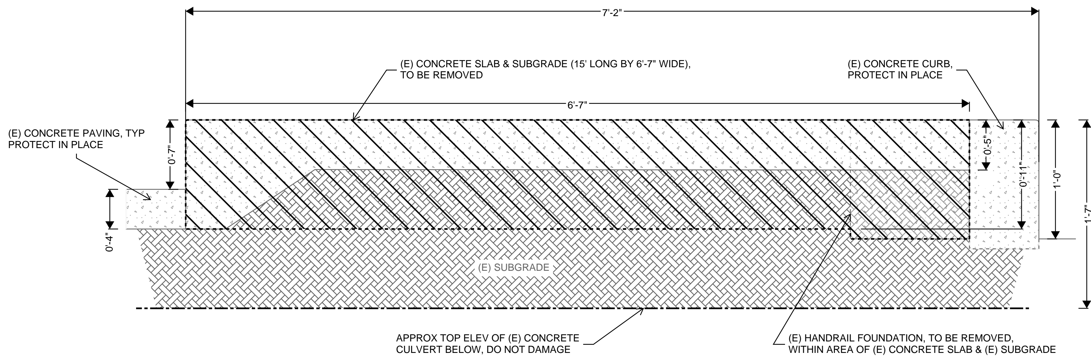
B C-6 SECTION C-C' - SLAB DEMOLITION (TYP) NTS
