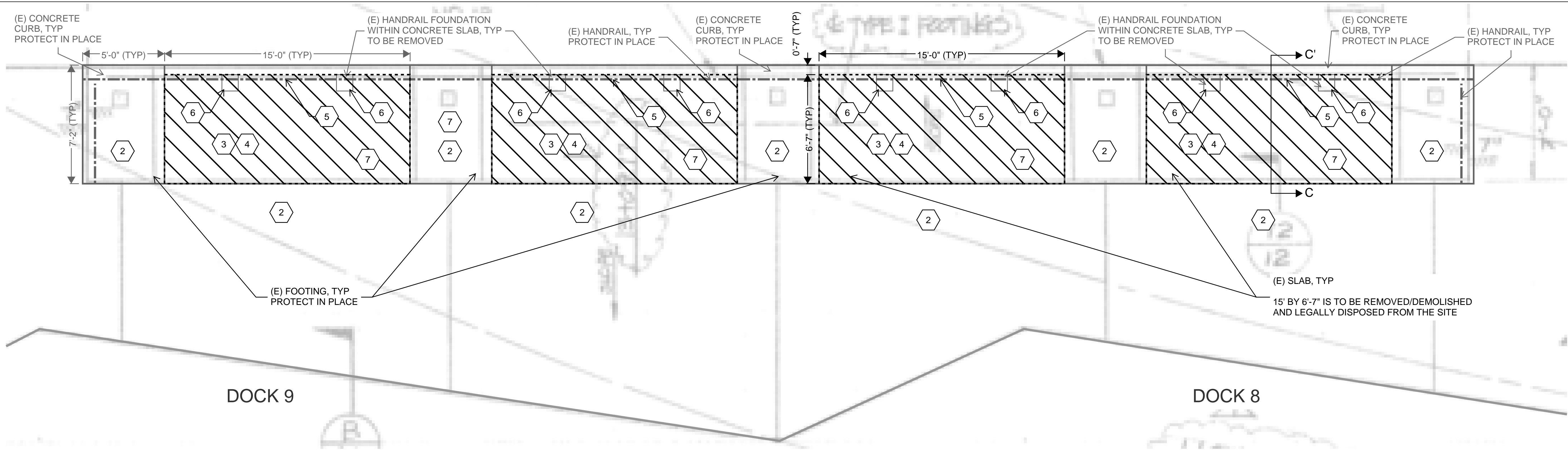
A C-6 RAISED PLATFORM - DEMOLITION PLAN NTS
