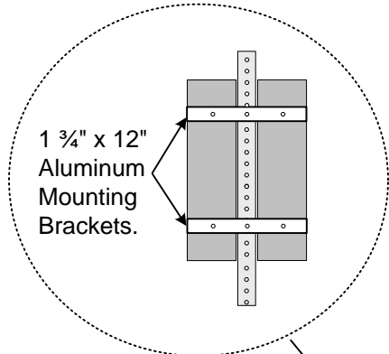
Rear View Mounting Detail
