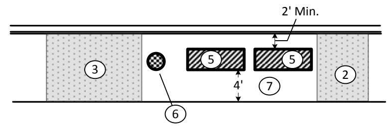
Alternate Bench Placement
