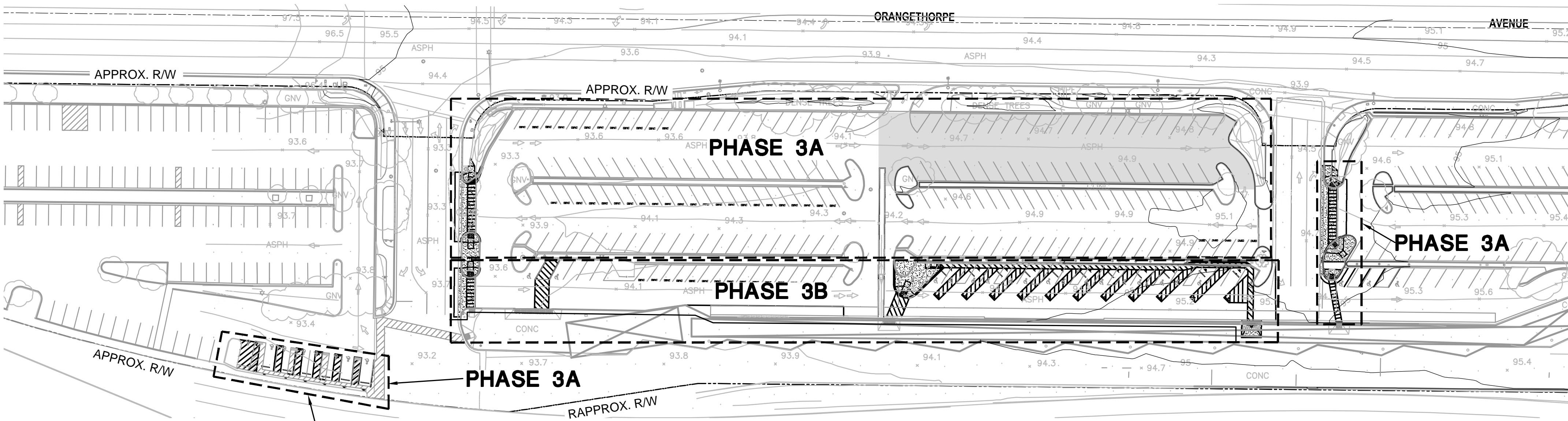
CONSTRUCTION PHASE 3 SCALE: 1" = 50'
