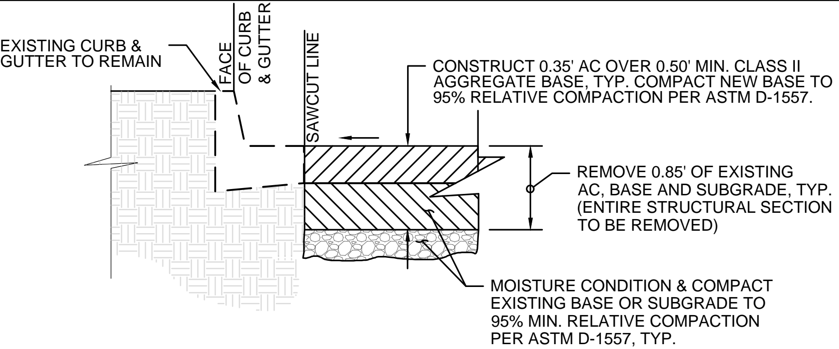
PAVEMENT RECONSTRUCTION SECTION A
