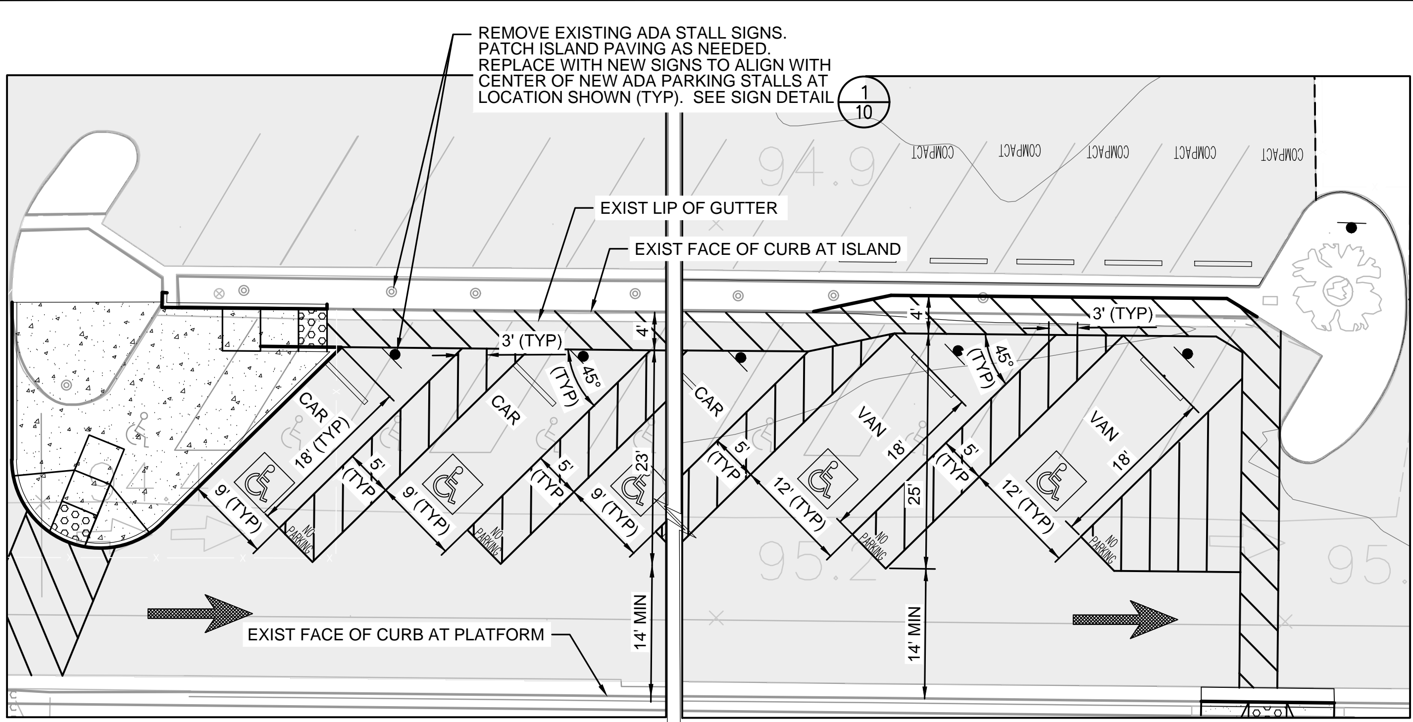
FULLERTON PARK AND RIDE TYPICAL ACCESSIBLE STALL DIMENSIONS
