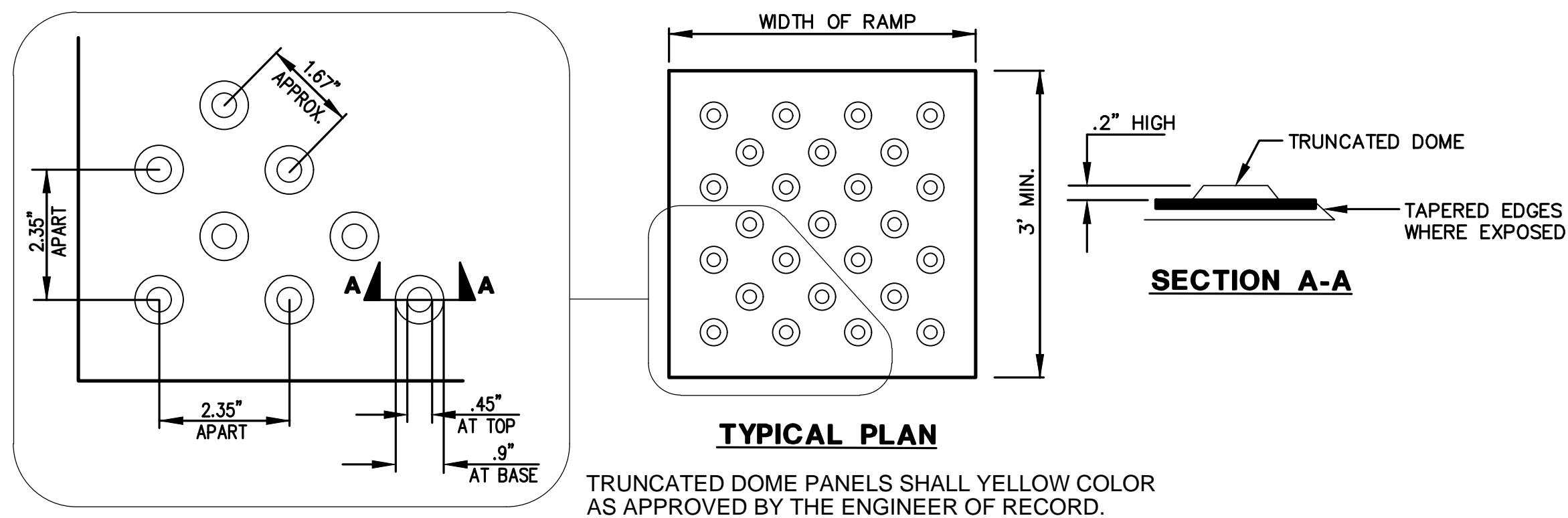
TRUNCATED DOME DETAIL 4 NTS
