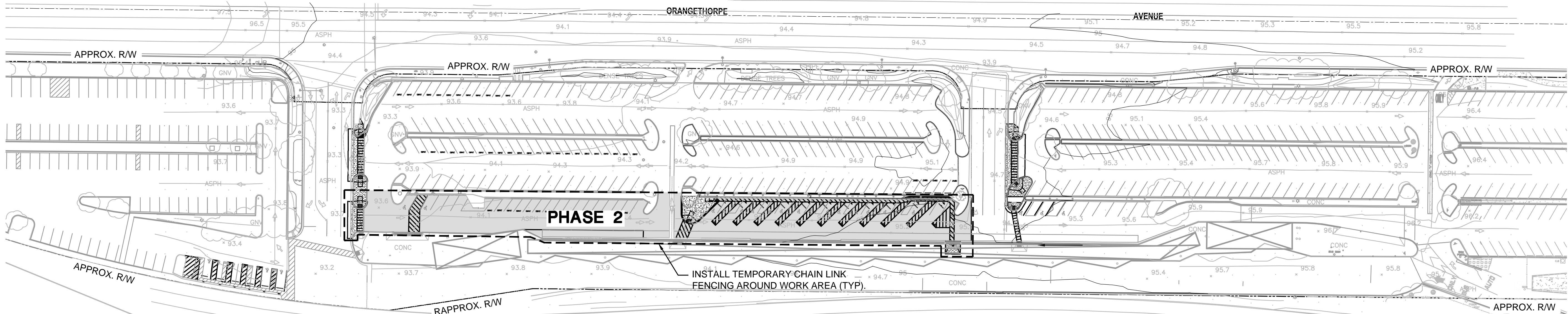
CONSTRUCTION PHASE 2 SCALE: 1" = 50'
