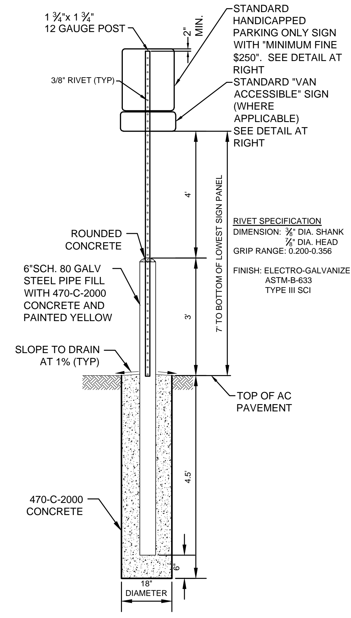
DETAIL 1 - NTS
